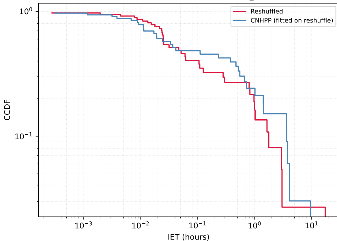
User 1025190273 - Reshuffled vs CNHPP A_{\text{fit}}=0.9327
